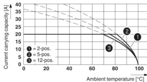
Derating curve for: PC 4/...-ST-7,62 with PCVK 4/...-G-7,62
